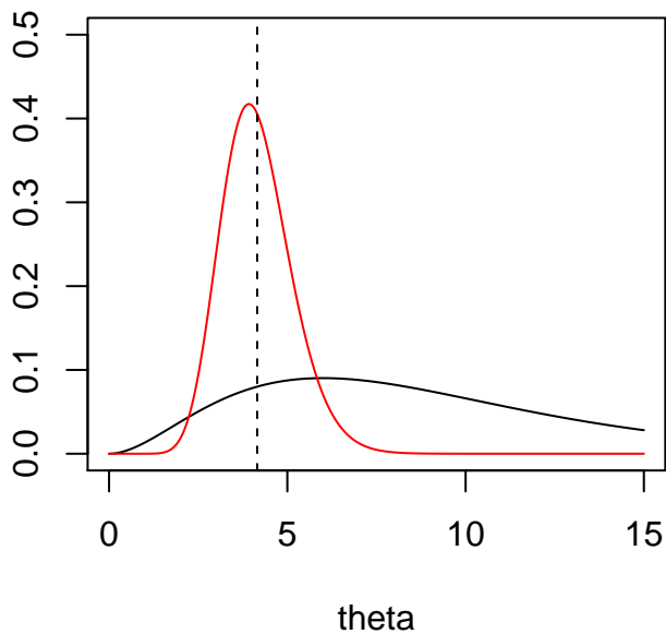
theta~Gamma(3,3)
