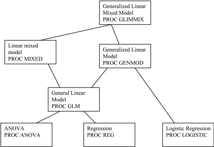
Figure 1. Linear Models Available in SAS/Stat
