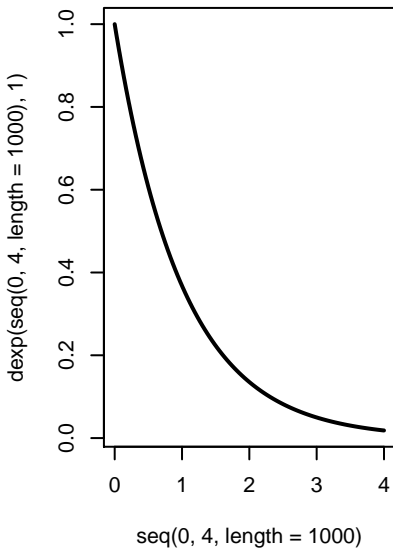
X~exp(1)
